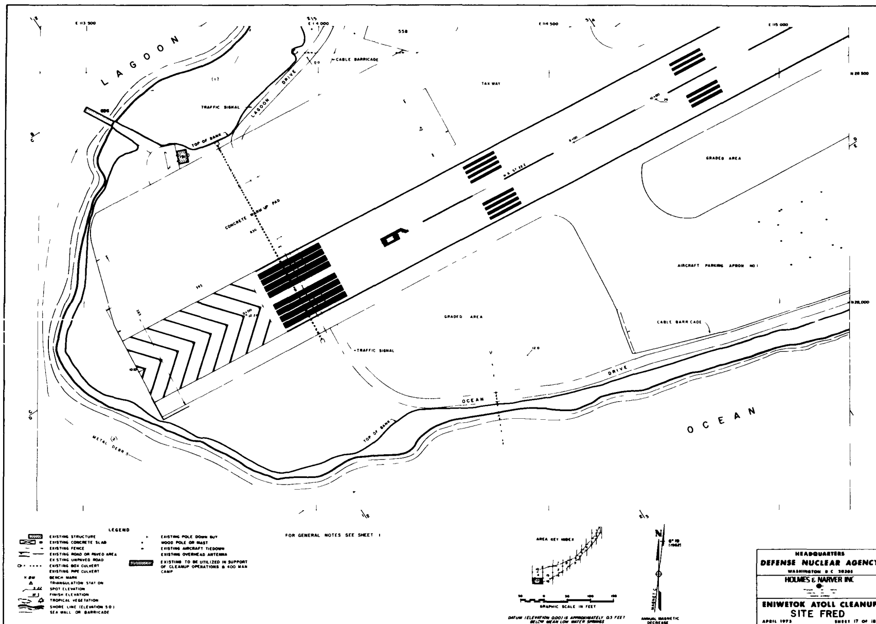
FIGURE 170 SITE FRED, SHEET 17 OF 18
